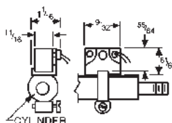
Pivot Extended (PE) 1-1/8", 1-1/2" & 2" bores only
