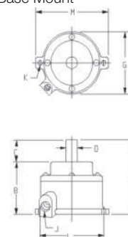
Base Mount
