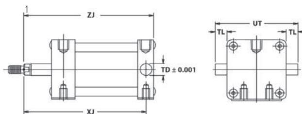
Blind End Trunnion Model TR
