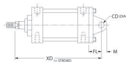
Long Clevis (PB)
