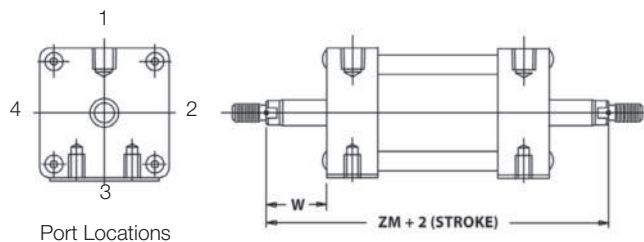
Double Rod Model DR
