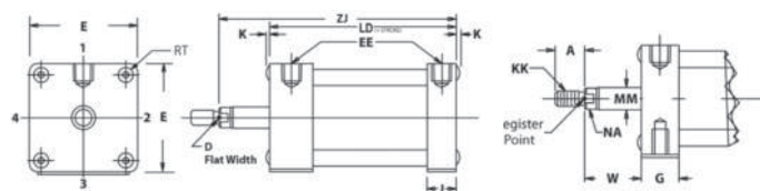
Basic Cylinder
