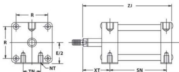
Rod End Trunnion Model TF
