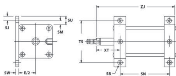
Foot Mount Plate Model FT
