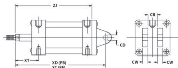
Clevis Model PB and PF
