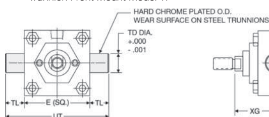
Trunnion Front Mount Model TF
