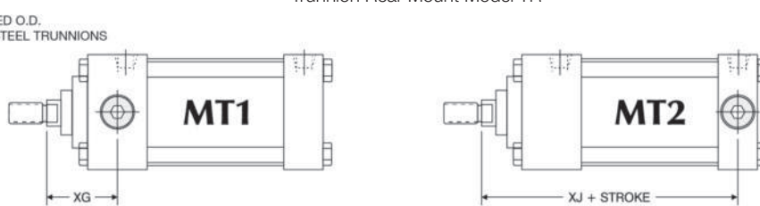
Trunnion Rear Mount Model TR
