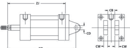
Clevis Model PB
