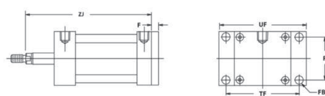
Blind End Flange Model FR*
