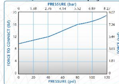
LQ4 Force to Connect Coupling
