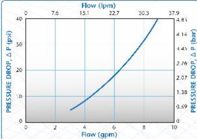
LQ4 Water Flow (0 – 20 GPM)
