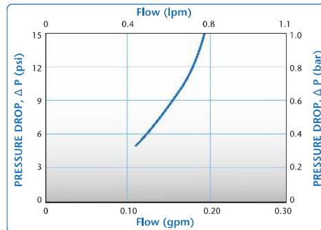
NS1 Water Flow
