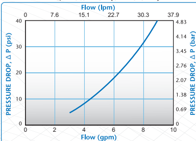
RPLQ4 Water Flow (0 – 20 GPM)
