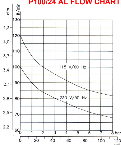
P100/24 AL FLOW CHART
