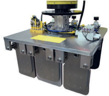
Carton Clamp
